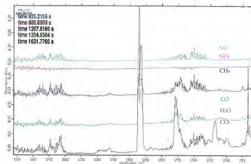
Figure 6. FTiR analysis of Jerusalem artichoke torrefaction by-products: torgas during the torrefaction process under 245 °C.
