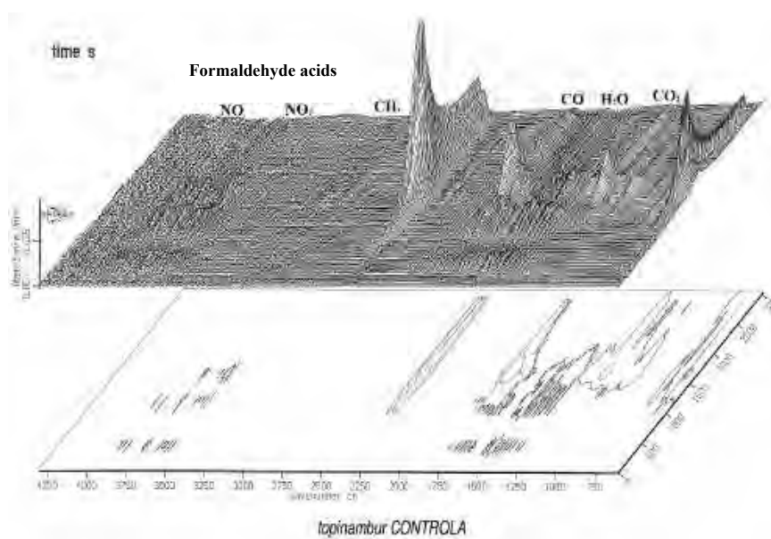
Figure 5. FTiR analysis of Jerusalem artichoke torrefaction by-products: torgas during the torrefaction process under 245 °C.
